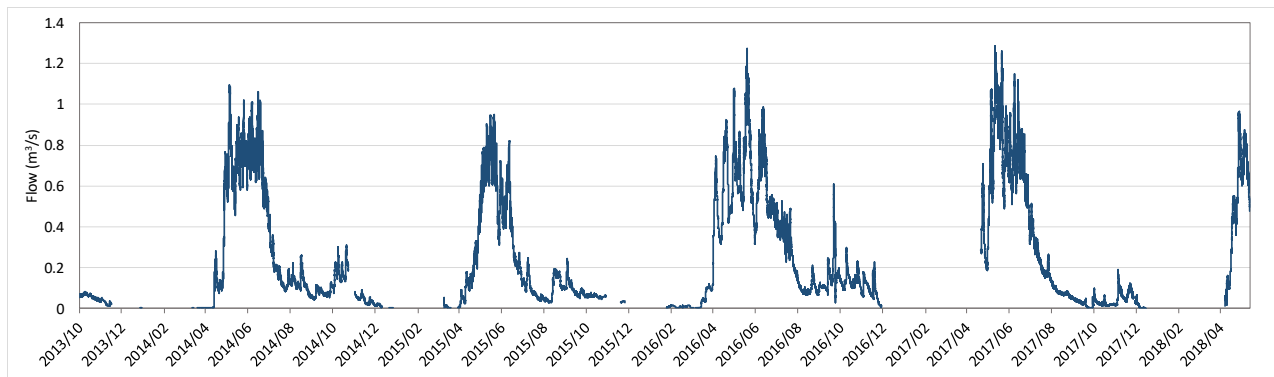
Figure 16. Discharge time-series data for Ben Hur Creek hydrometric station.
