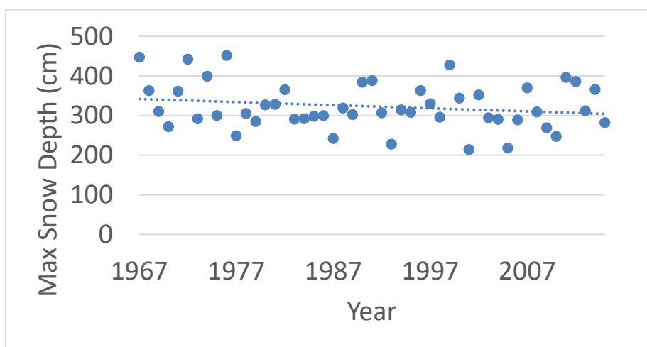
Figure 37. Annual maximum snow depth measured at the St. Leon snow course.
