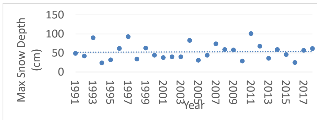
Figure 36. Annual maximum snow depth measured at two BC snow courses situated below 1600 m elevation in Representative Area: a) Sandon b) Duncan Lake No.2.
