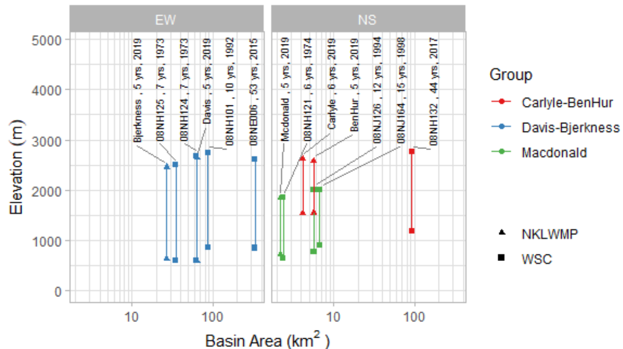
Figure 44. Dominant valley orientation (EW=East-West, NS=North-South) and elevation range for the NKLWMP and WSC watersheds. Each station is labelled with station name/number, number of years on record, and year of last recorded data.
