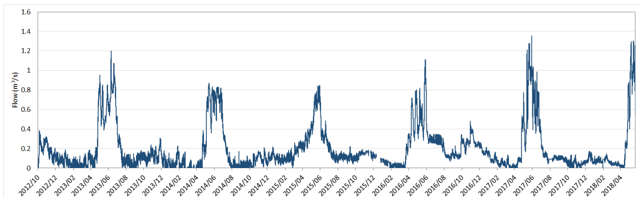
Figure 15. Discharge time series for Carlyle Creek hydrometric station.
