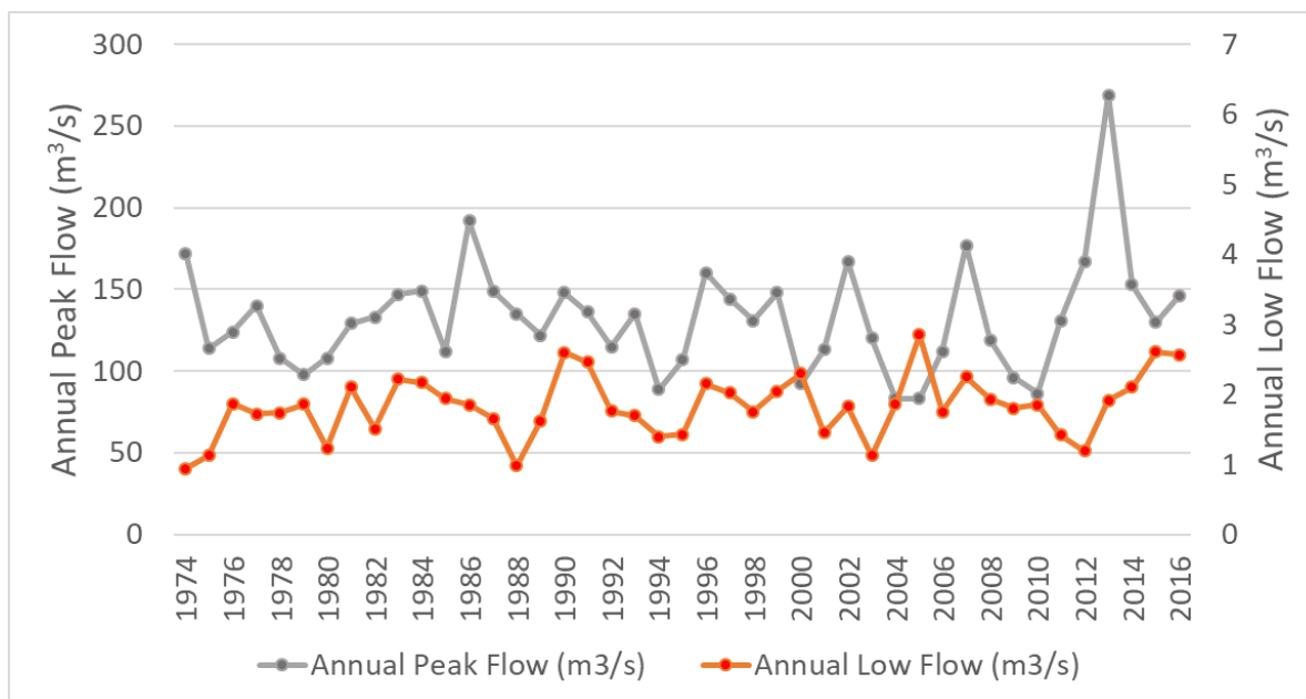
Figure A6.1. Peak-flow and low-flow time-series for Fry Creek below Carney Creek (WSC 08NH130) during period of record.
