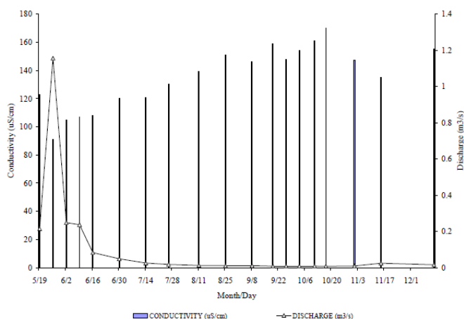
Figure 11. Discharge and conductivity versus in 1999 for MacDonald Creek (from Quamme and Sundberg 2000).
