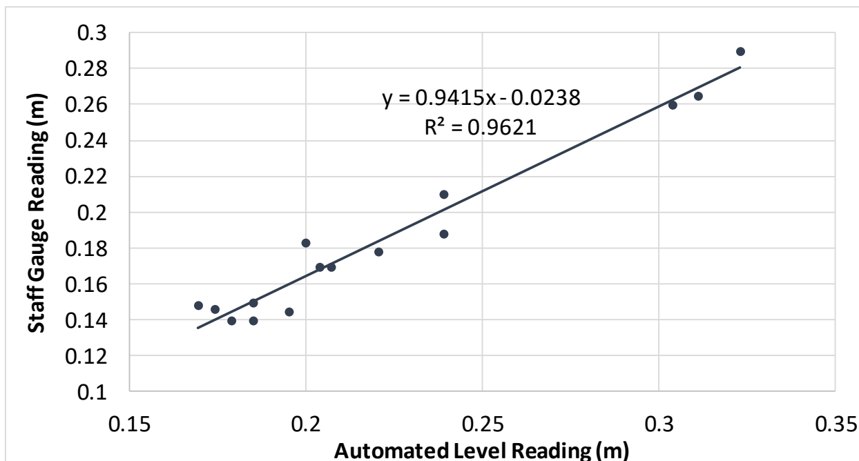
Figure A3.5. Relation between automated (data logger) and manual (staff gauge) level readings at the MacDonald hydrometric station.
